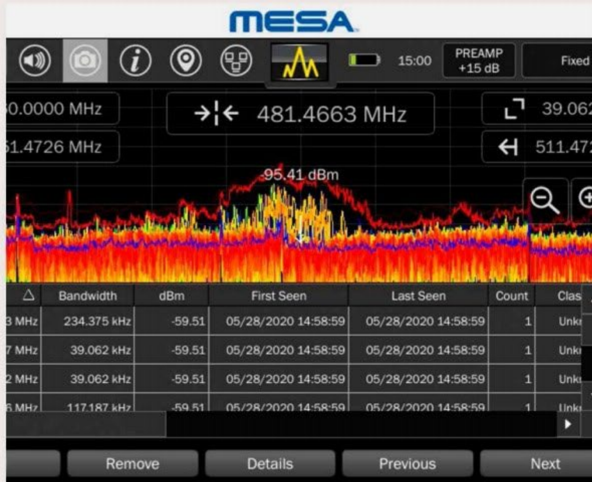
Spectrum Analyzer with Signal List
